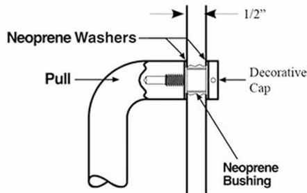
Thru Bolt for Glass Door
