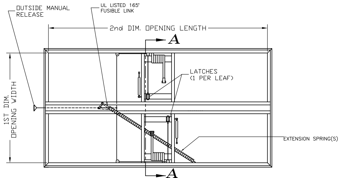
PLAN VIEW COVERS REMOVED
